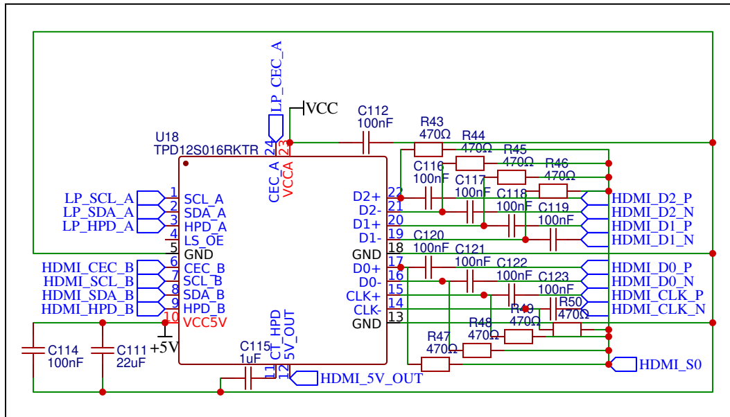
HDMI Port
